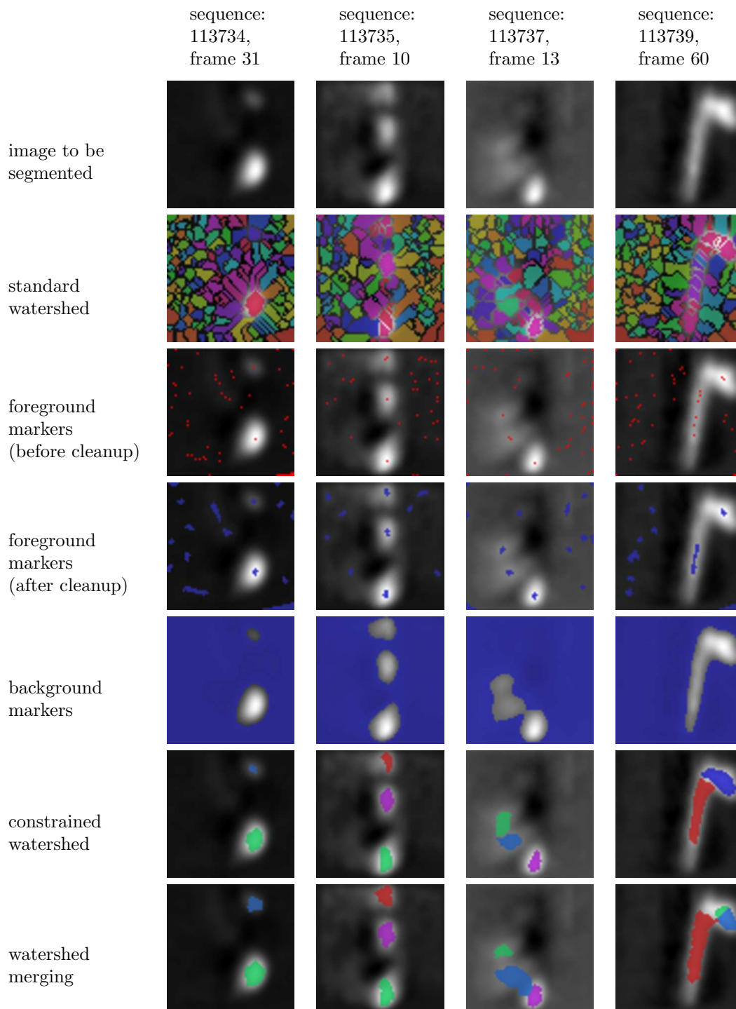
Figure 4. Results for watershed segmentation. Row 1 - image to be segmented; row 2 - standard watershed segmentation indicating the over-segmentation of the image; row 3 - foreground markers obtained without the cleanup step; row 4 - foreground markers obtained after the cleanup step; row 5 - background markers; row 6 - constrained watershed segmentation; row 7 - results with watershed merging
