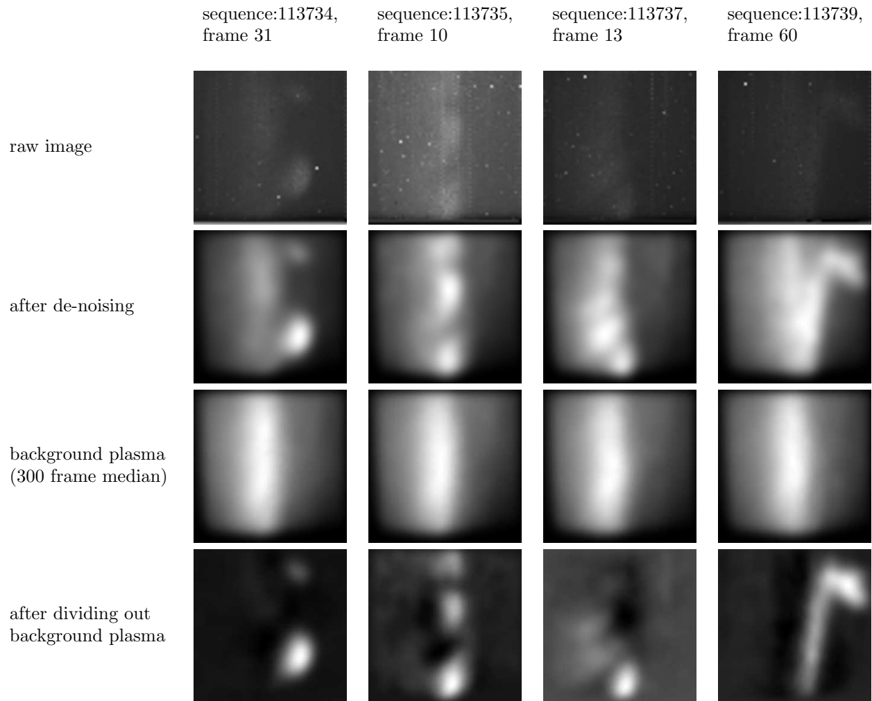
Figure 1. Removal of noise and background plasma from the raw image data for 4 frames from 4 different sequences. First row: original images. Second row: after filtering to remove noise. Third row: the quiescent or background plasma, defined as the median of the 300 frames of each sequence. Fourth row: Filtered image after the quiescent plasma intensity has been divided out.
