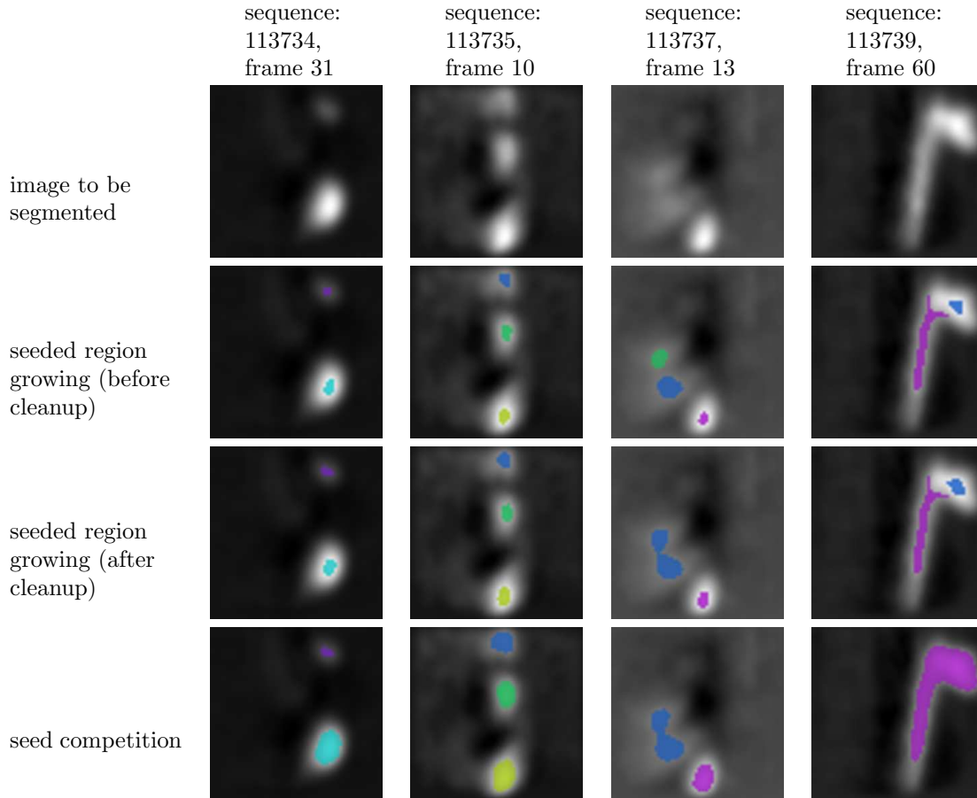
Figure 5. Results from the seeded region growing and seed competition methods: Row 1 - image to be segmented; row 2 - results of seeded region growing from foreground markers before cleanup (Figure 4 row 3); row 3 - results of the seeded region growing from foreground markers after cleanup (Figure 4 row 4); row 4 - results from the seed competition method.
