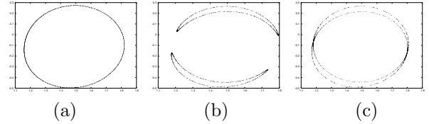
Figure 2: An example of an orbit from each class. (a) Quasi-periodic. (b) Island chain with two islands. (c) Separatrix with two cross points.
